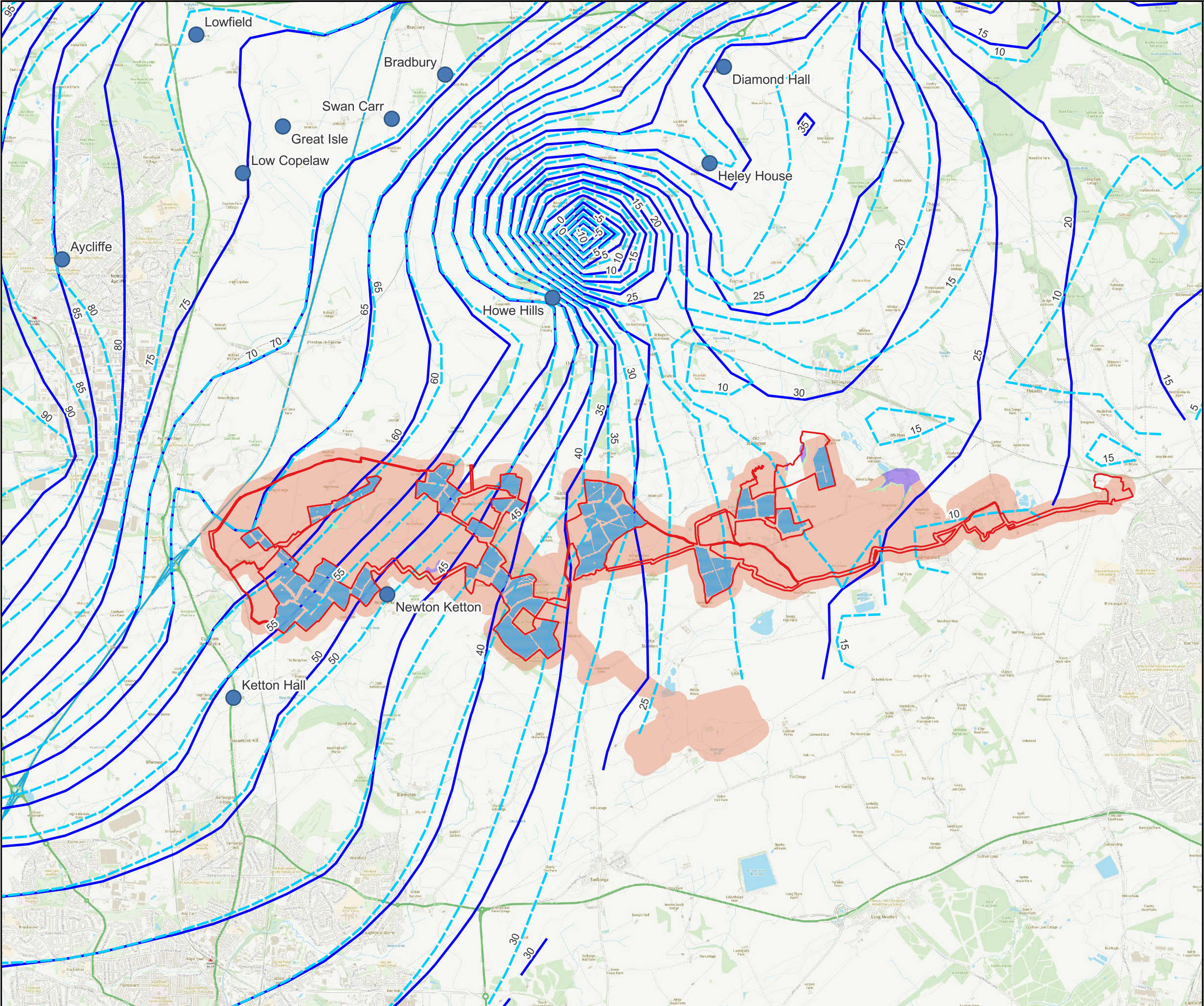
Drawing Title Figure 5.1 Groundwater Contours
